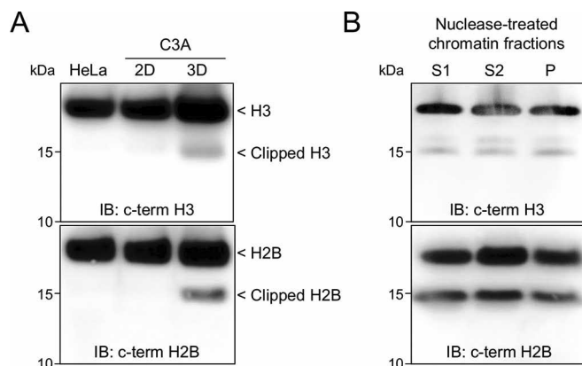
FIG. 1. Histones H3 and H2B undergo proteolytic processing in 3D cell culture. A, C3A cell line cultured as a flat culture (2D) or as a spheroid culture (3D) and HeLa cell line (2D) were harvested and protein extracts were analyzed by immunoblotting (IB) using the antibodies indicated in each panel. B, Chromatin isolated from 21 days old 3D C3A cell culture was partially digested with MNase and subsequently fractionated into euchromatin (S1), heterochromatin (S2) and matrix-associated chromatin (P) subfractions. Resulting protein fractions were analyzed by immunoblotting.
