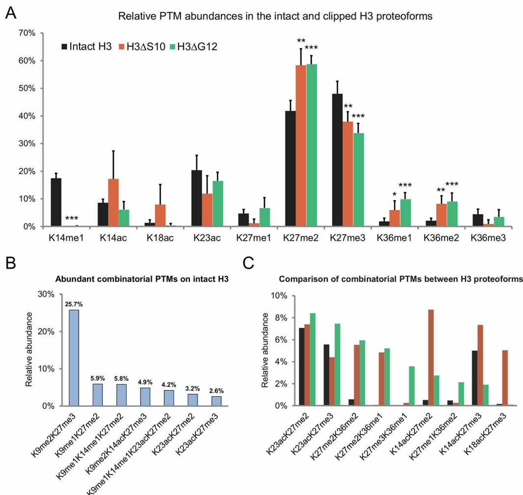
FIG. 4. Clipped histone H3 proteoforms contain PTMs with significantly different relative abundance as compared with intact H3. A, Relative abundances of the ten most abundant individual PTMs in the intact and clipped H3 proteoforms identified by middle-down MS/MS analysis. The relative abundance of each individual modification was calculated as the sum of relative abundances of all distinct PTM peptide forms containing this particular modification. Different H3 proteoforms are indicated by color in the top of the panel. The same colors for different H3 proteoforms are used in bar plot (C). Data are means \pm s.d. ( n = 6 ). Asterisk indicates differentially abundant PTMs (* ( p < 0.05 ), ** ( p < 0.005 ), and *** ( p < 0.0005 )). B, Relative abundances of the seven most frequently observed combinatorial marks identified in N-terminal tail of intact H3. C, Relative abundances of the nine most frequently observed combinatorial marks identified in N-terminal tails of clipped H3ΔS10 and H3ΔG12 proteoforms. The frequencies of these combinatorial marks in intact H3 were calculated as a sum of the frequency of the combinatorial PTM in intact H3 and frequencies of all combinatorial PTMs containing this PTM pair in combination with any of modifications of K4 and K9 (e.g. the frequency of K14acK27me2 was calculated as a sum of frequencies of K14acK27me2, K9me1K14acK27me2, and K9me3K14acK27me2).
