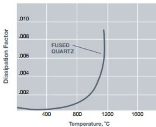
Dissipation Factor
