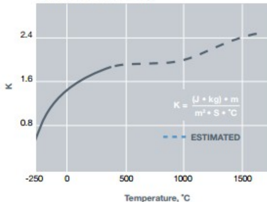
Thermal Conductivity
